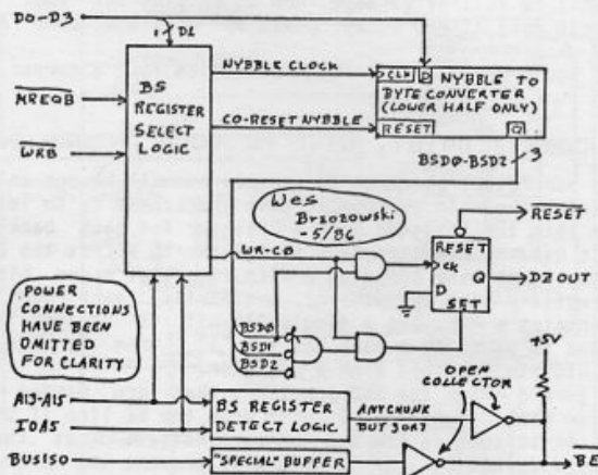
FIG 3. BEU FUNCTIONS TO ADD BUSISO & DZOUT
